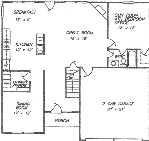
FIRST FLOOR — FLOOR PLAN
