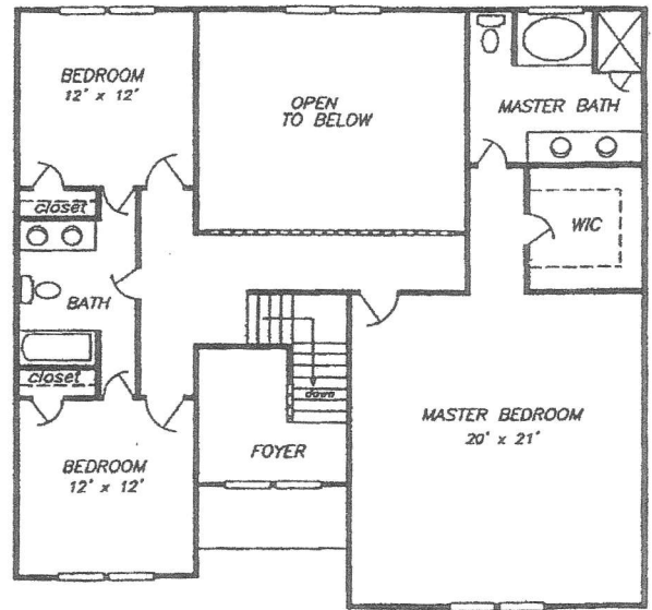
SECOND FLOOR — FLOOR PLAN
